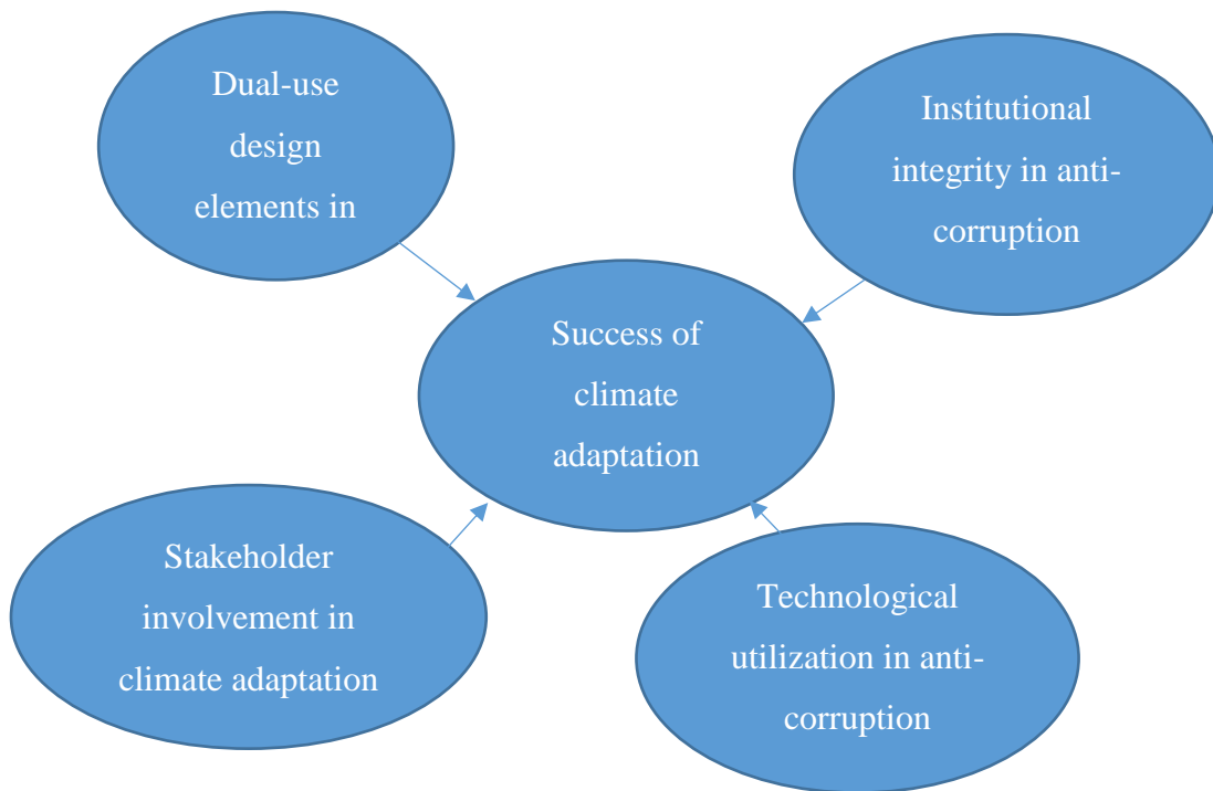
Fig 1: Theoretical Framework
